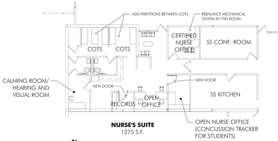
NURSE'S SUITE 1275 S.F. NEW WORK FLOOR PLAN SCALE: 1/8" = 1'-0"
